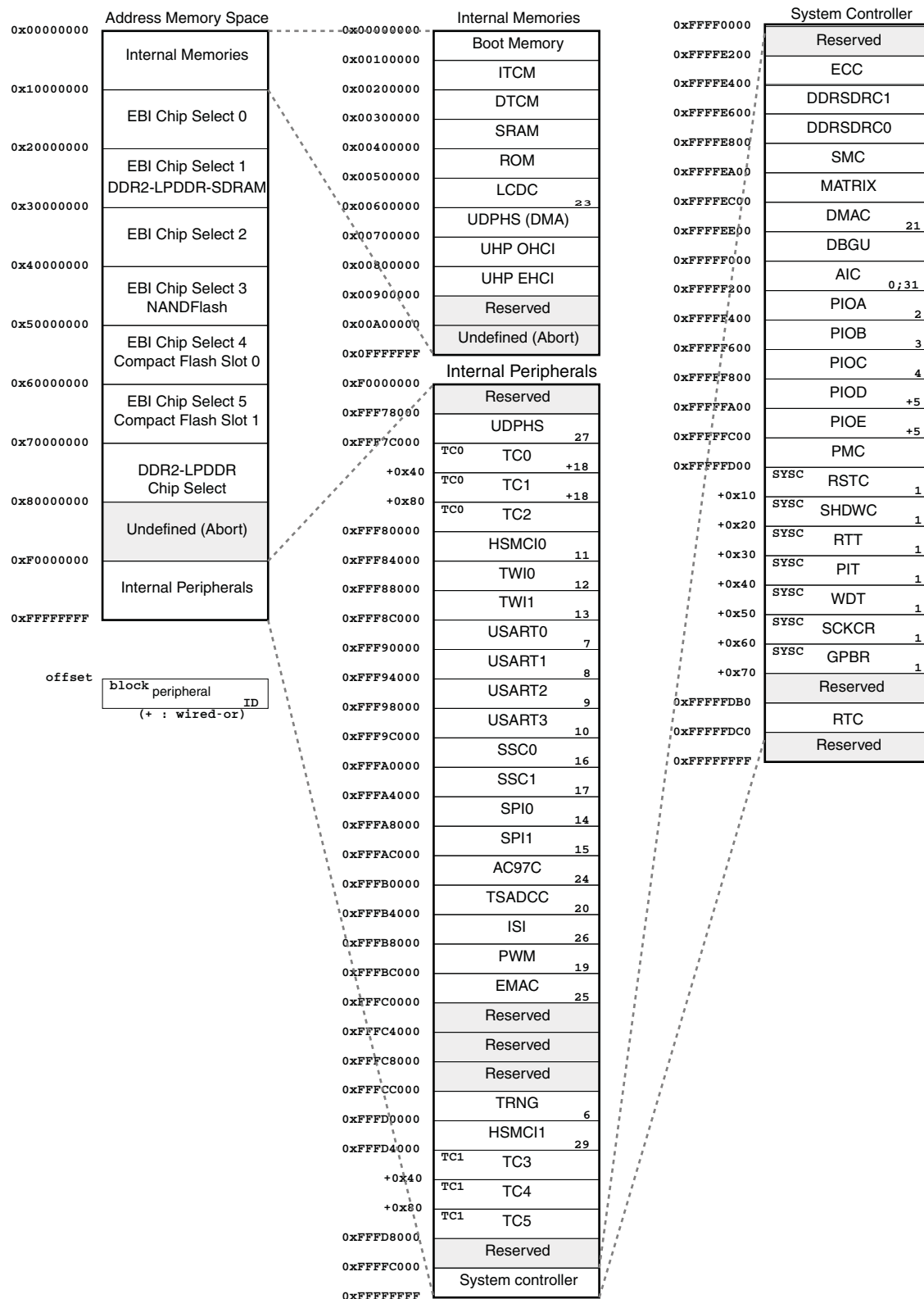
Figure 6-1. AT91SAM9G45 Memory Mapping
