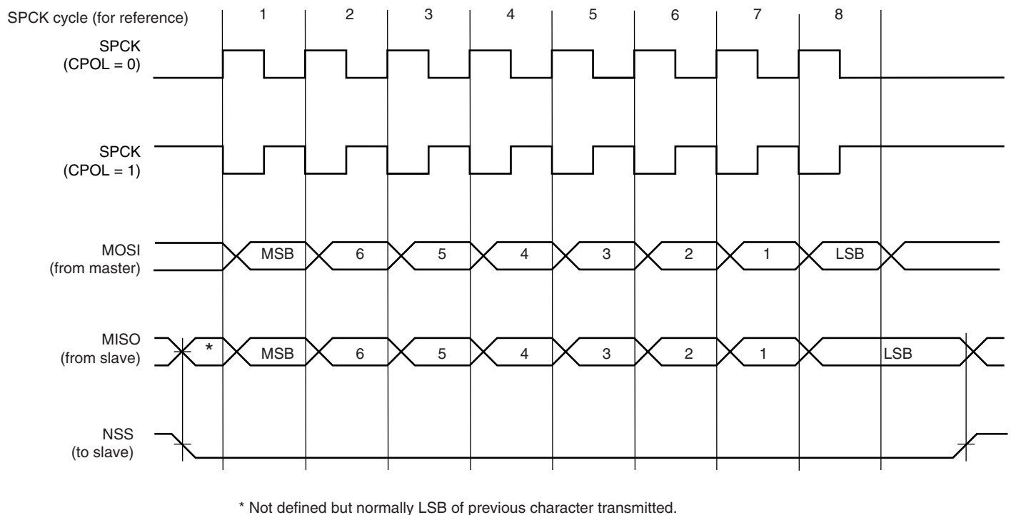
Figure 30-5. SPI Transfer Format (NCPHA = 0, 8 bits per transfer)
